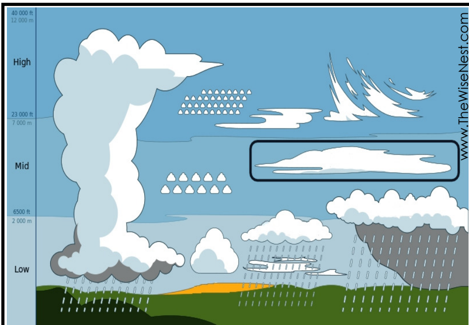
altostratus
