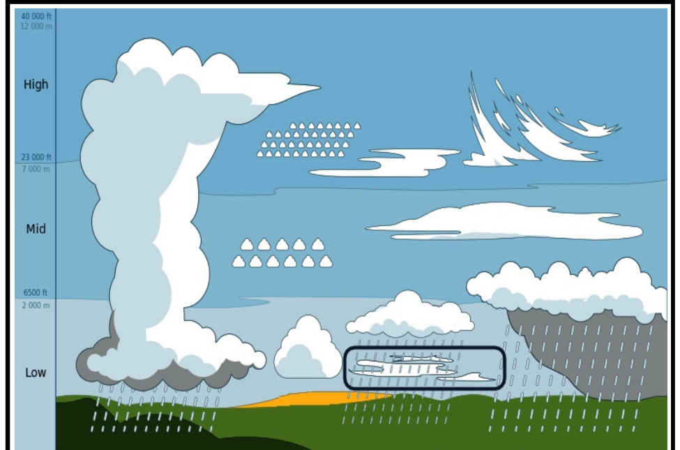
stratus
