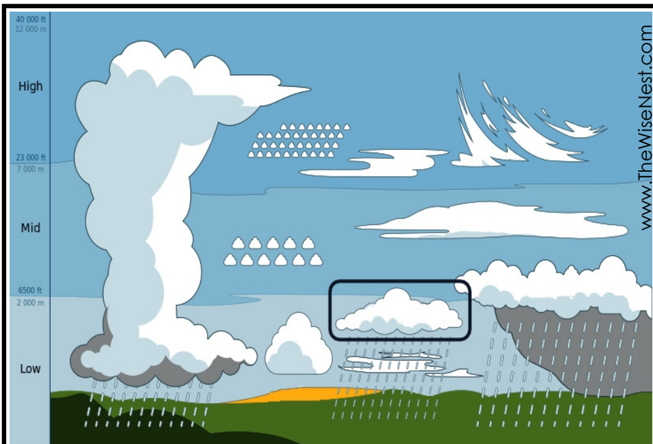
stratocumulus
